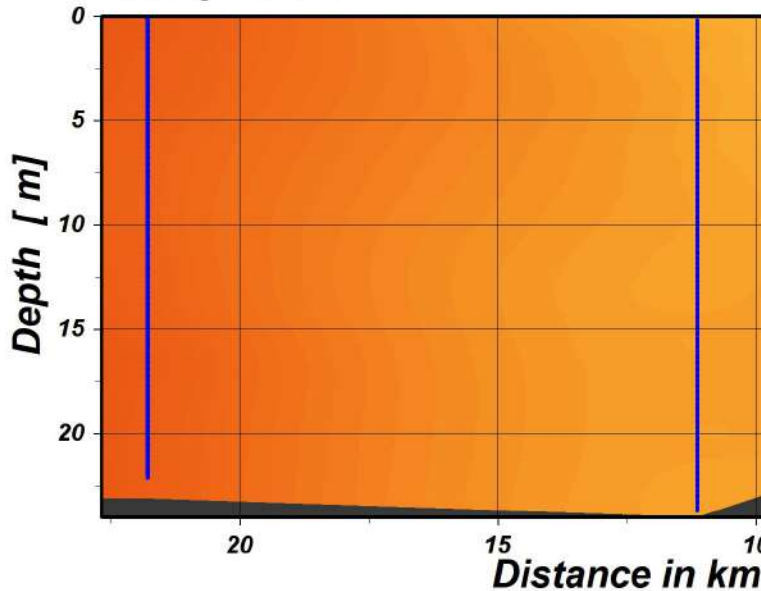
Salinity - isolines
