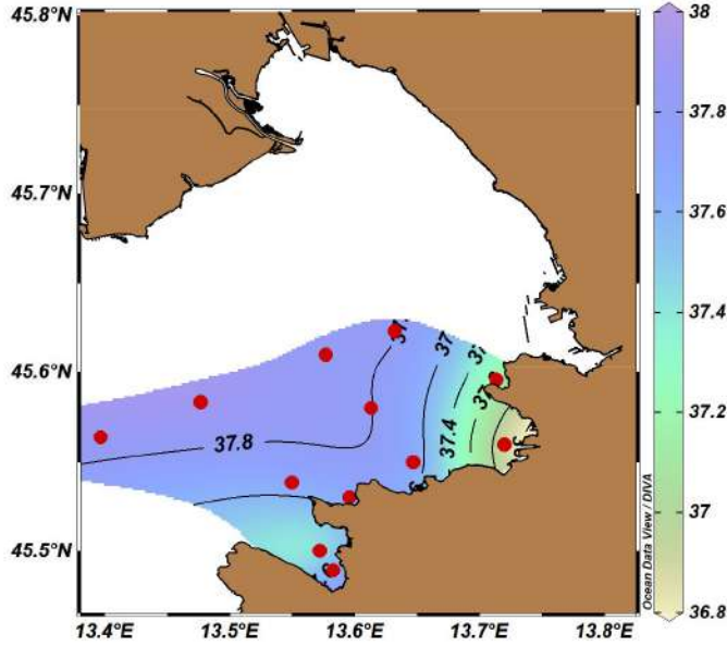
Surface Salinity
