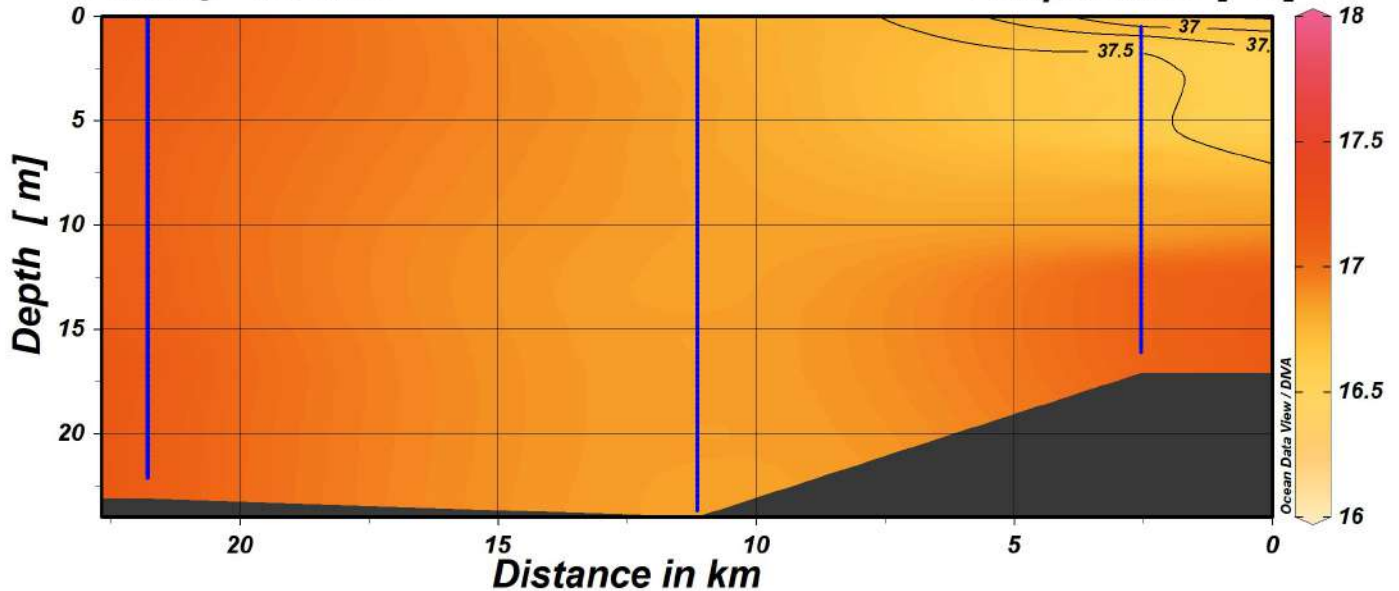
Salinity - isolines
