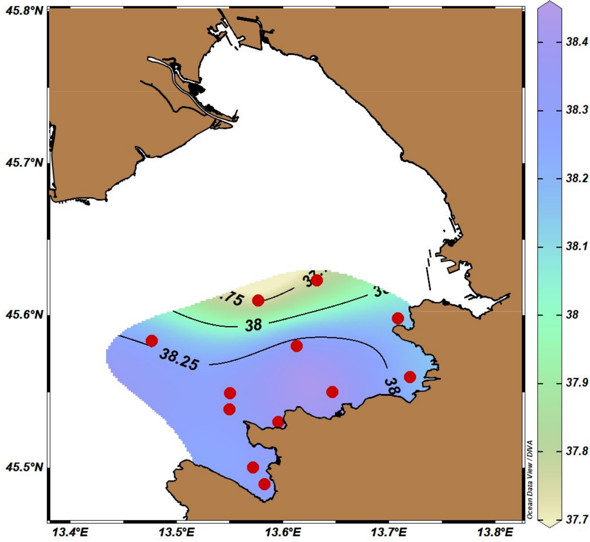
Surface Salinity
