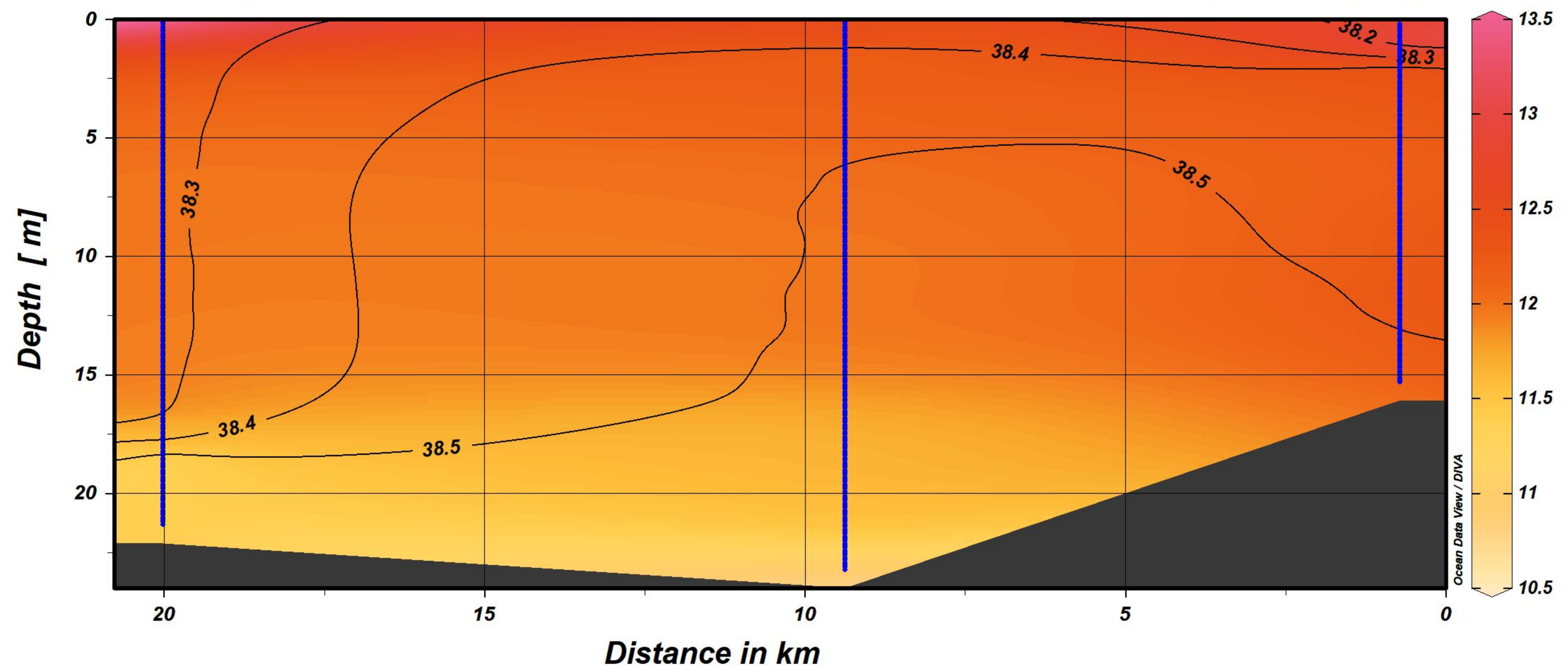
Salinity - isolines
