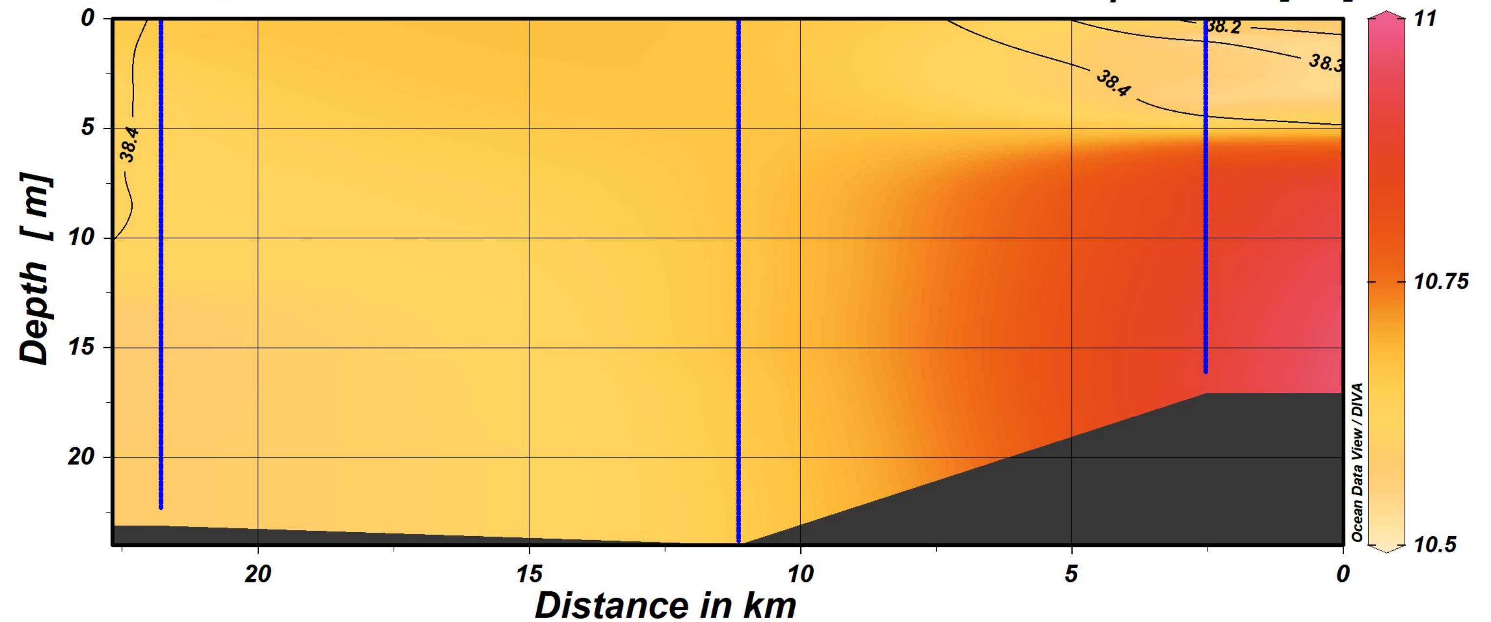
Salinity - isolines
