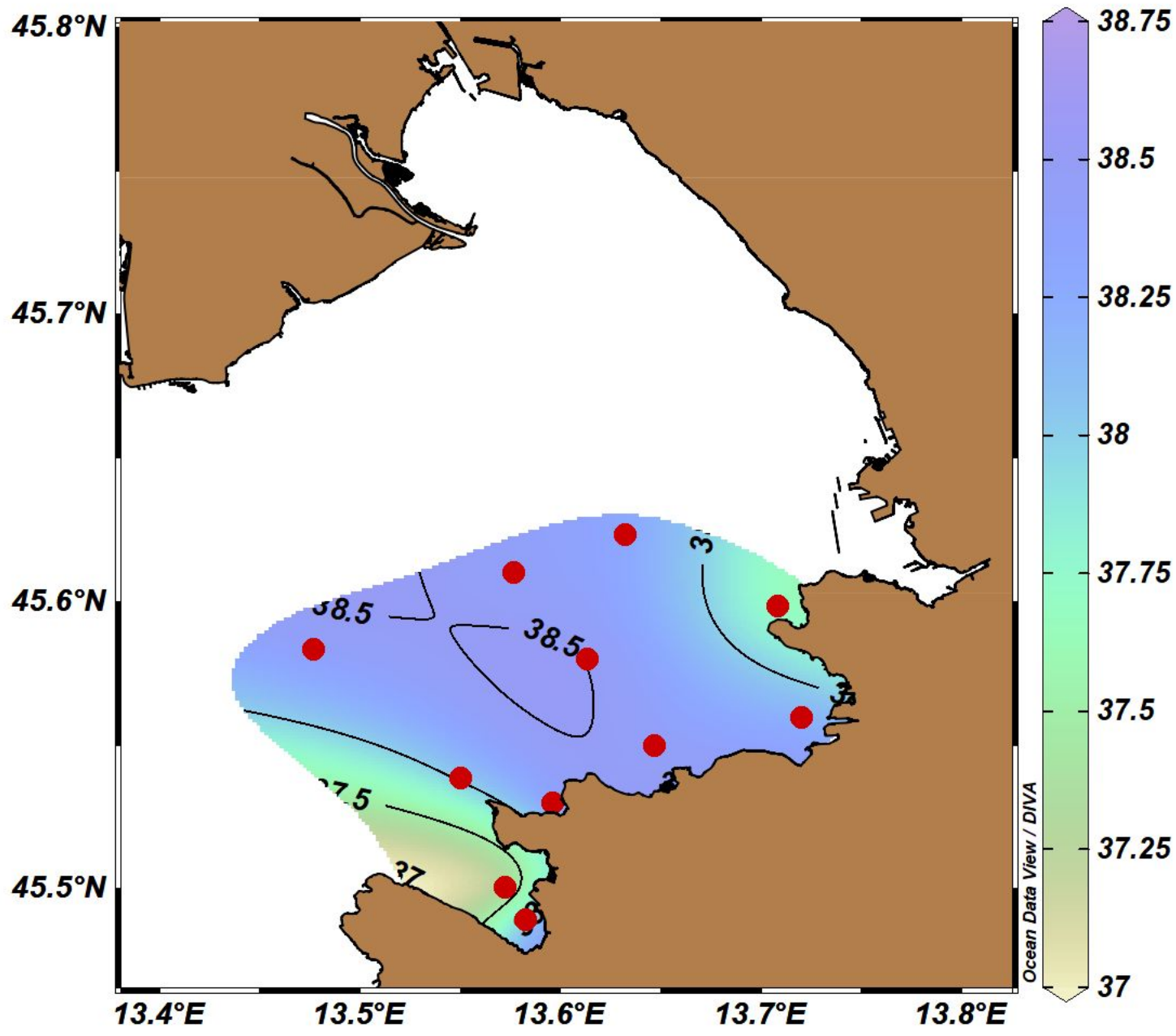
Surface Salinity
