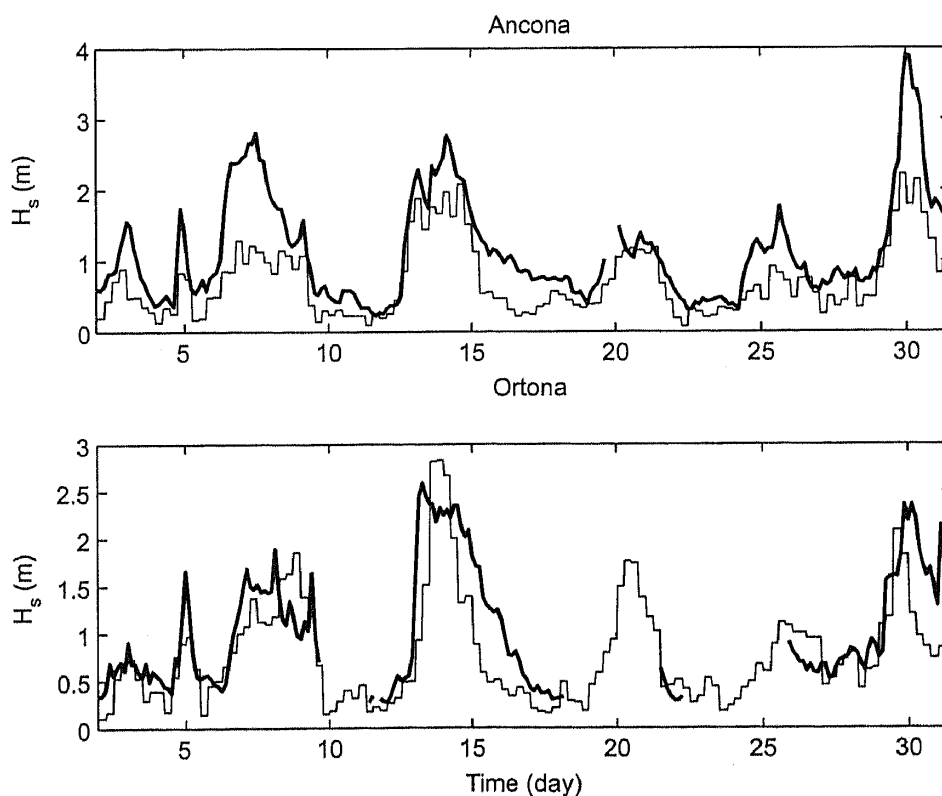
Fig. 4. Comparison of hourly significant wave height predicted by SWAN (thin line) and 3-h measurements (thick line) at Ancona ( 43^{\circ}37.00'\text{N} , 13^{\circ}51.00'\text{E} ) and Ortona ( 42^{\circ}24.07'\text{N} , 14^{\circ}32.04'\text{E} ).
