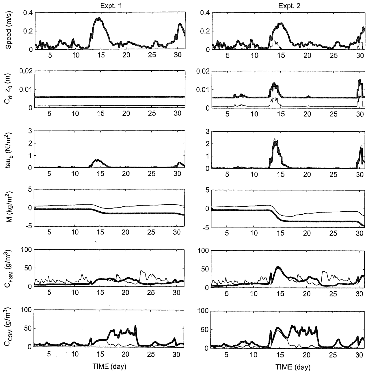
Fig. 5. The hourly time series of BBL hydrodynamics properties, bed load, and sediment concentrations in January 2001 at station S1 predicted by Experiment 1 (left) and Experiment 2 (right). From top: the bottom mean current (thick line) and bottom wave orbital velocity (thin line); the bottom roughness z_0 (thin line) and drag coefficient C_d (thick line); bottom stress \tau_b predicted by Experiments 1 and 2 (thick line) and Experiment 3 (thin line); sedimentation (bed load M ) for FSM (thick line) and CSM (thin line); FSM concentration C_{fsm} at surface (thin line) and bottom (thick line); CSM concentration C_{csm} at surface (thin line) and bottom (thick line). Bed load is the time integration of the bottom sediment flux due to deposition and resuspension.
