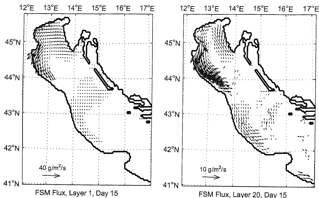
Fig. 10. Model simulated horizontal FSM fluxes at surface (layer 1) and bottom (layer 20) on 15 January 2001, by Experiment 1. Vectors less than 30% of maximum fluxes are not plotted.
