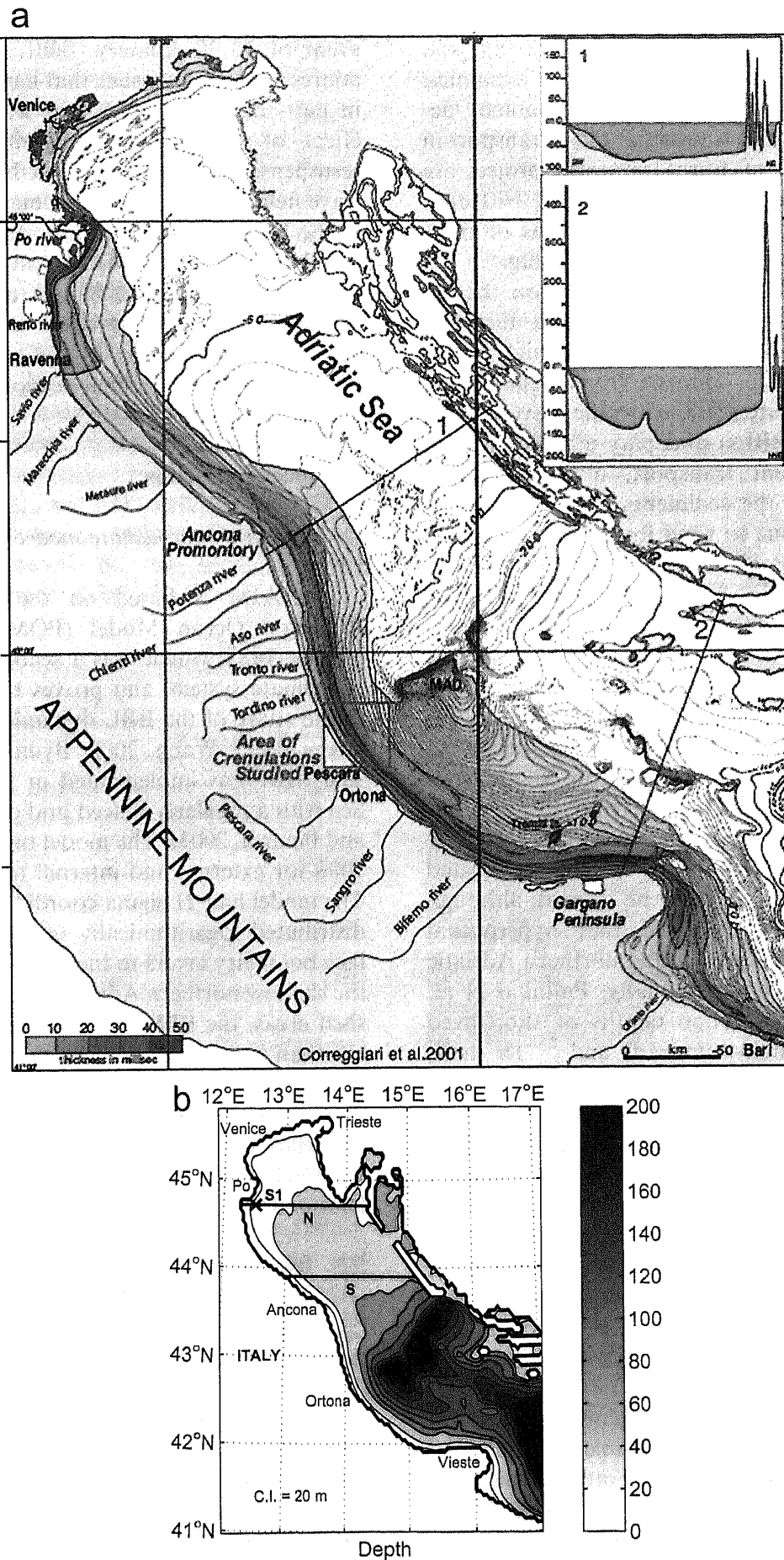
Fig. 1. (a) The northern Adriatic Sea bathymetry and Holocene sediment depositions. Figure from Correggiari et al. (2001); (b) the NAS model domain. S1 denotes location for station S1. N and S denote two cross-sections south of the Po River delta, and near Ancona, respectively.
