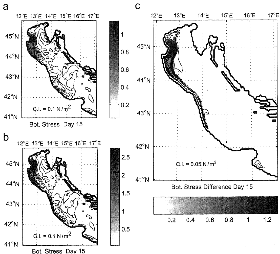
Fig. 6. The bottom stress on 15 January 2001, predicted by Experiment 1 (a), Experiment 2 (b), and their difference (c).
