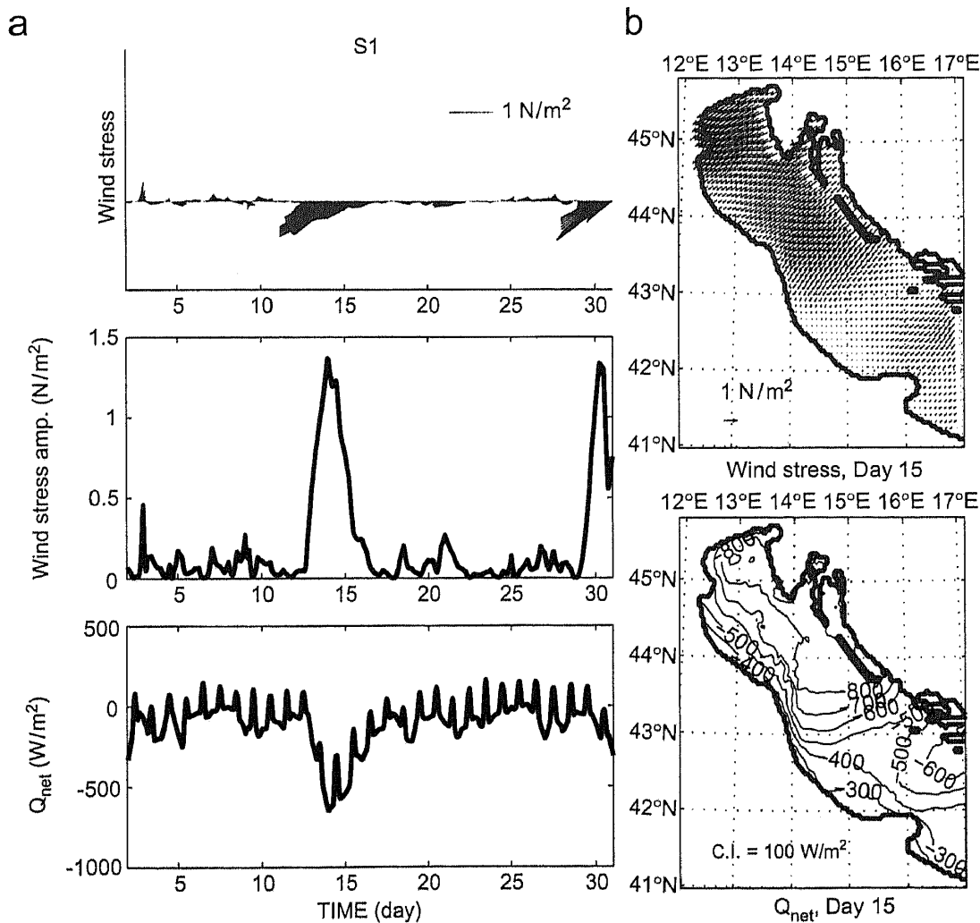
Fig. 2. (a) January 2001 wind stress and net surface heat flux at station S1. The European Centre for Medium Range Weather Forecast (ECMWF) 6-h analysis wind fields were used for the wind stress computation. The wind stress vectors were on the conventional geographical coordinate system. The ECMWF and COADS (Comprehensive Ocean Atmosphere Data Set) data were used to compute the surface heat flux with the bulk aerodynamic formulae. (b) ECMWF wind stress and net surface heat flux over the northern Adriatic Sea on 15 January 2001.
