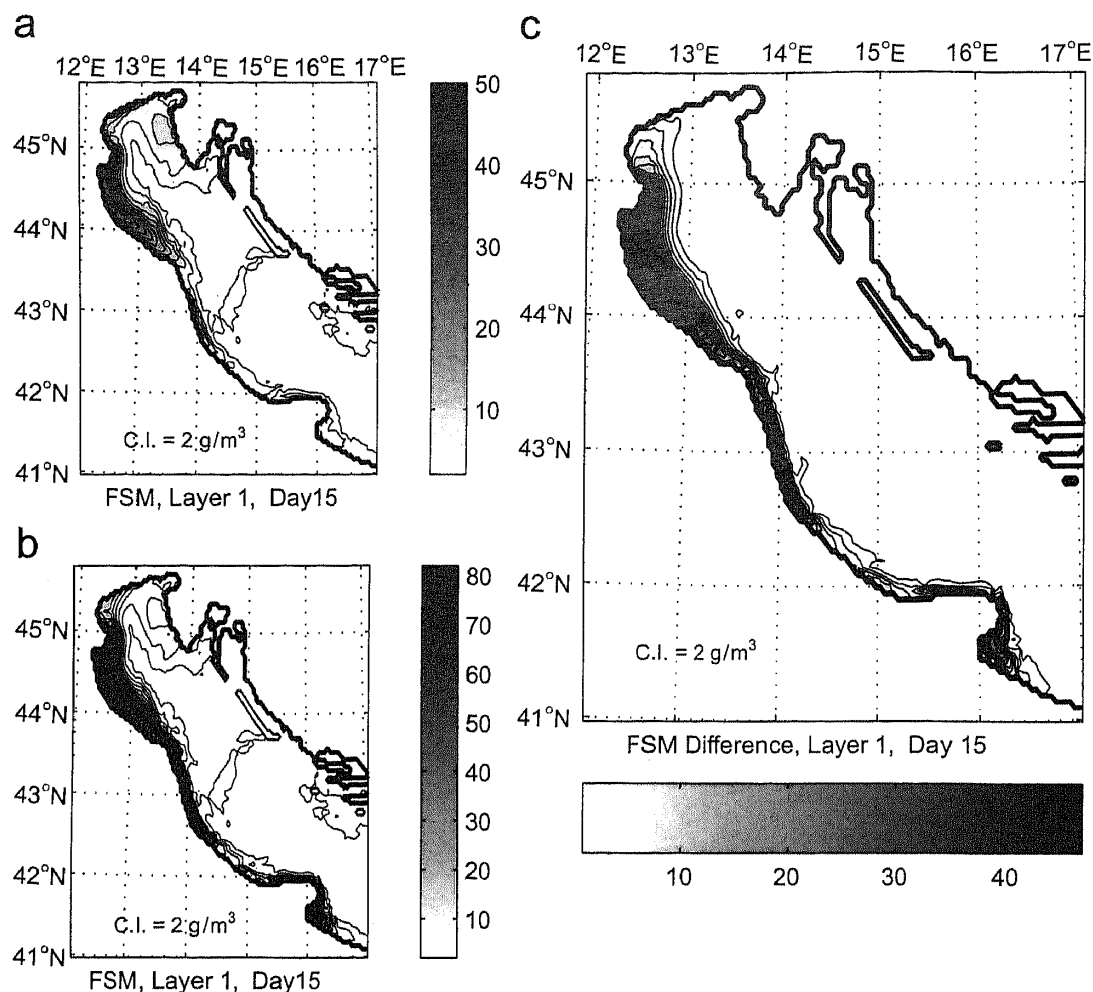
Fig. 7. The surface (layer 1) FSM concentration on 15 January 2001, predicted by experiment 1 (a), Experiment 2 (b), and their difference (c).
