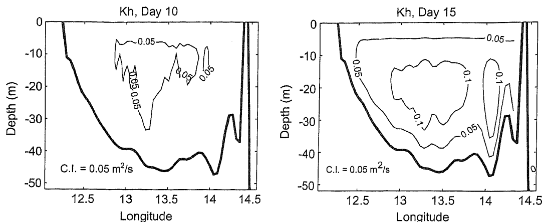
Fig. 9. Model simulated vertical eddy diffusivity at cross section N on 10 and 15 January 2001, by Experiment 1.
