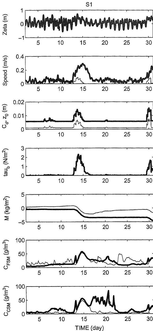
Fig. 12. The same as Fig. 5 but predicted by Experiment 4. The surface elevation at S1 is also shown in the top panel.
