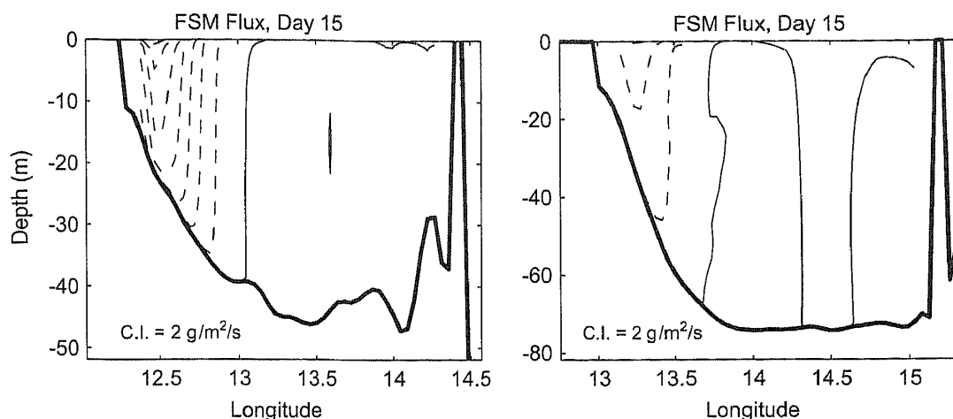
Fig. 11. Model simulated horizontal FSM fluxes at cross section N (left) and cross section S (right) on 15 January 2001, by Experiment 1.
