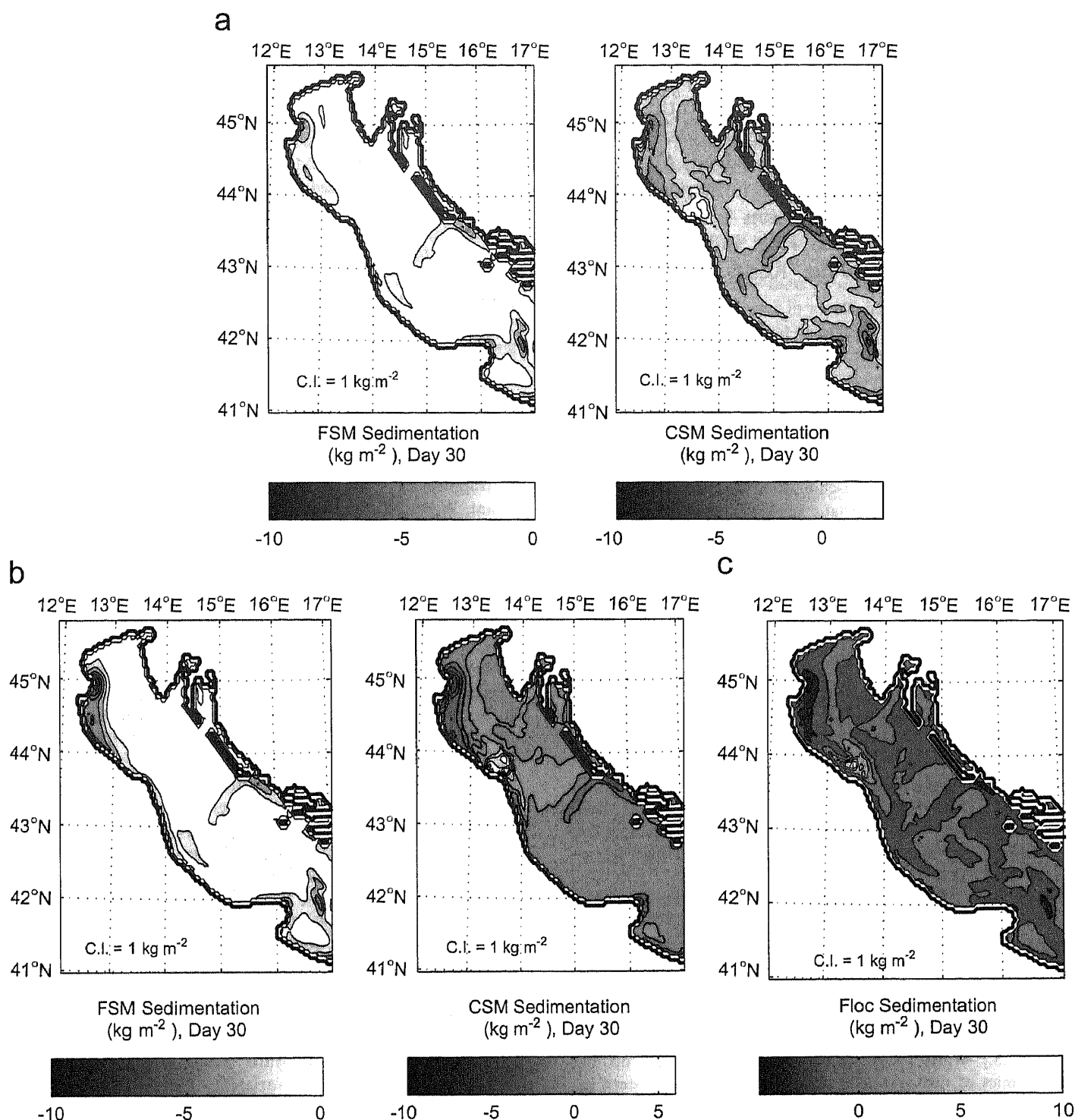
Fig. 13. Model simulated monthly net sedimentation by (a) Experiment 1; (b) Experiment 2, and (c) Experiment 2, but w_s = -10^{-3} \text{ m s}^{-1} .
