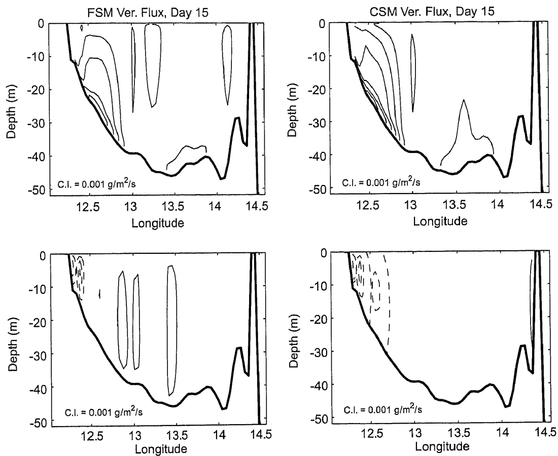
Fig. 8. Model simulated vertical FSM and CSM fluxes at cross section N on 15 January, 2001, by experiment 1. Top: -K_h(\partial C/\partial z) ; bottom: (w+w_s)C . Downward fluxes are in negative values denoted by the dashed lines.
